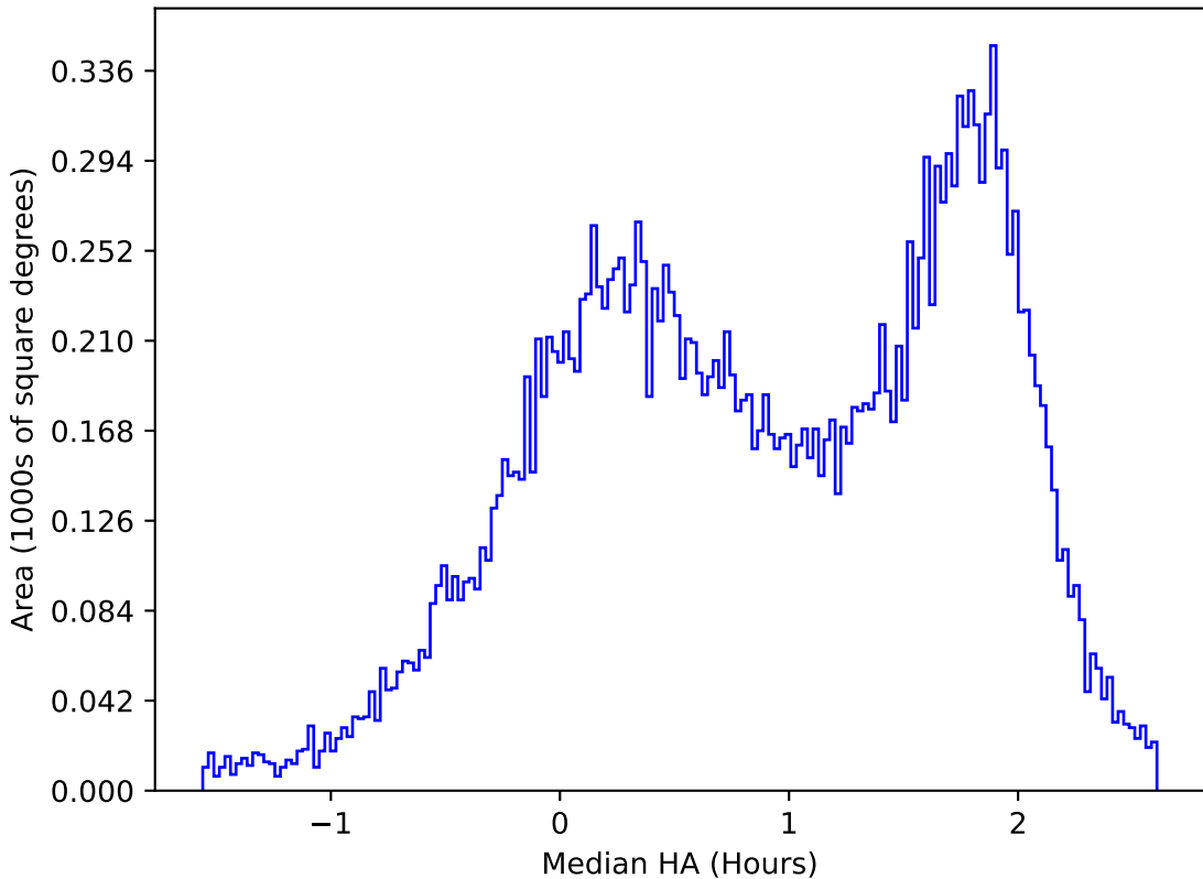
ddf_acor_sf10_ls40_lsr50_v3.4_10yrs All sky u band: Median HA
