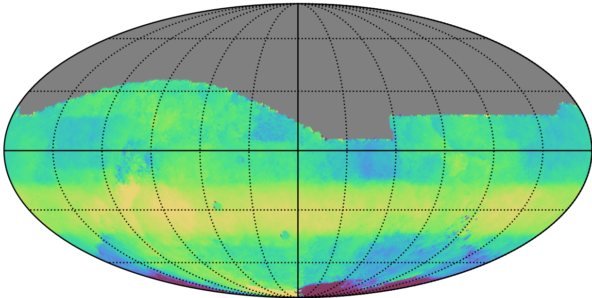
ddf_acor_sf10_lsf40_lsr50_v3.4_10yrs All sky r band: Median HA
