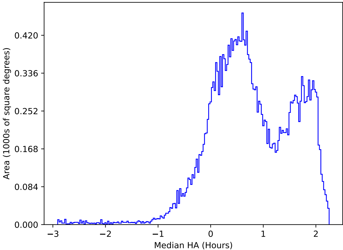
ddf_acor_sf10_lsf40_lsr50_v3.4_10yrs All sky r band: Median HA
