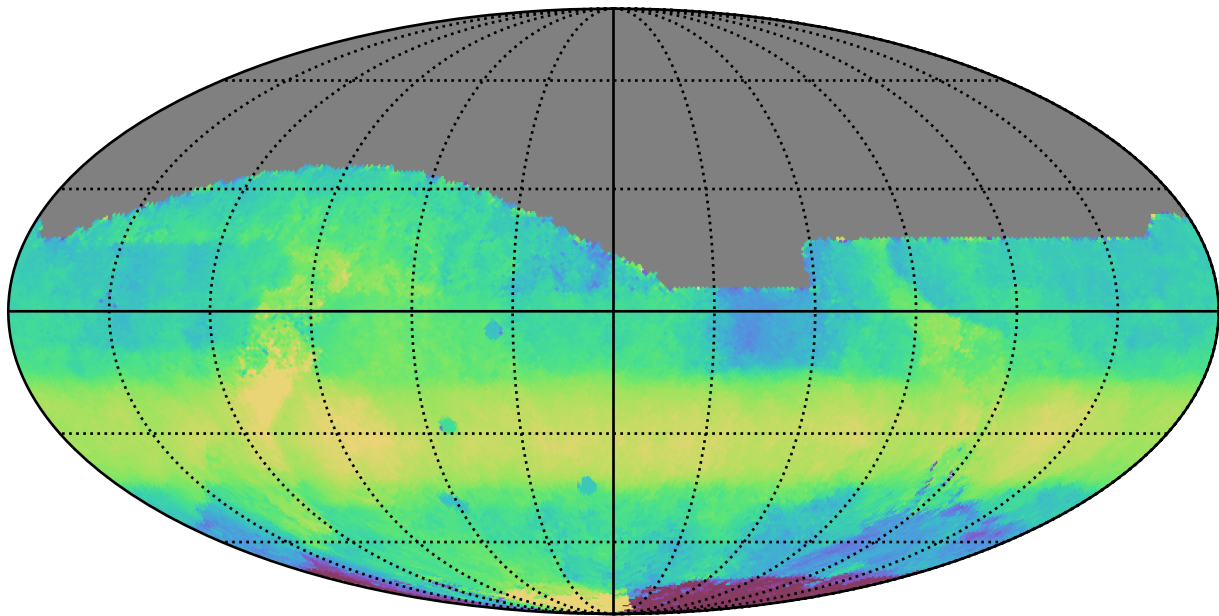
ddf_acor_sf10_lsf40_lsr50_v3.4_10yrs All sky i band: Median HA
