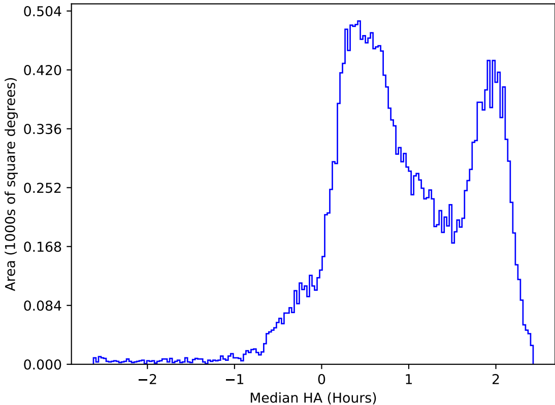
ddf_acor_sf10_lsf40_lsr50_v3.4_10yrs All sky i band: Median HA
