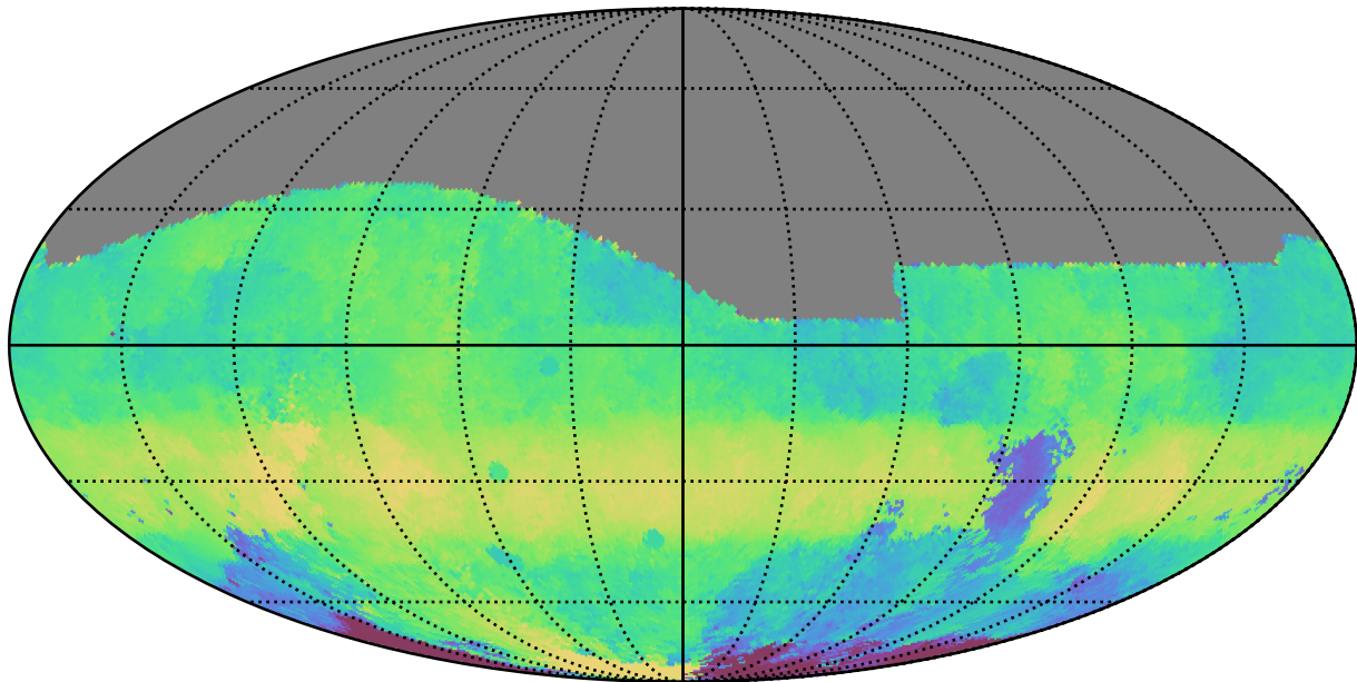
ddf_acor_sf10_lsf40_lsr50_v3.4_10yrs All sky g band: Median HA
