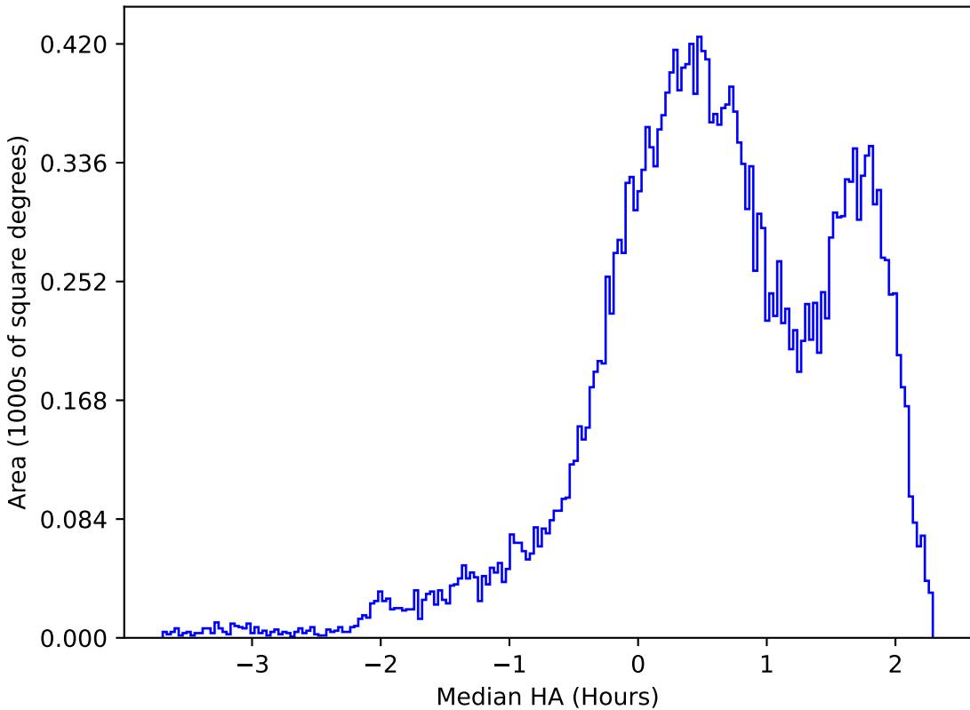
ddf_acor_sf10_lsf40_lsr50_v3.4_10yrs All sky g band: Median HA
