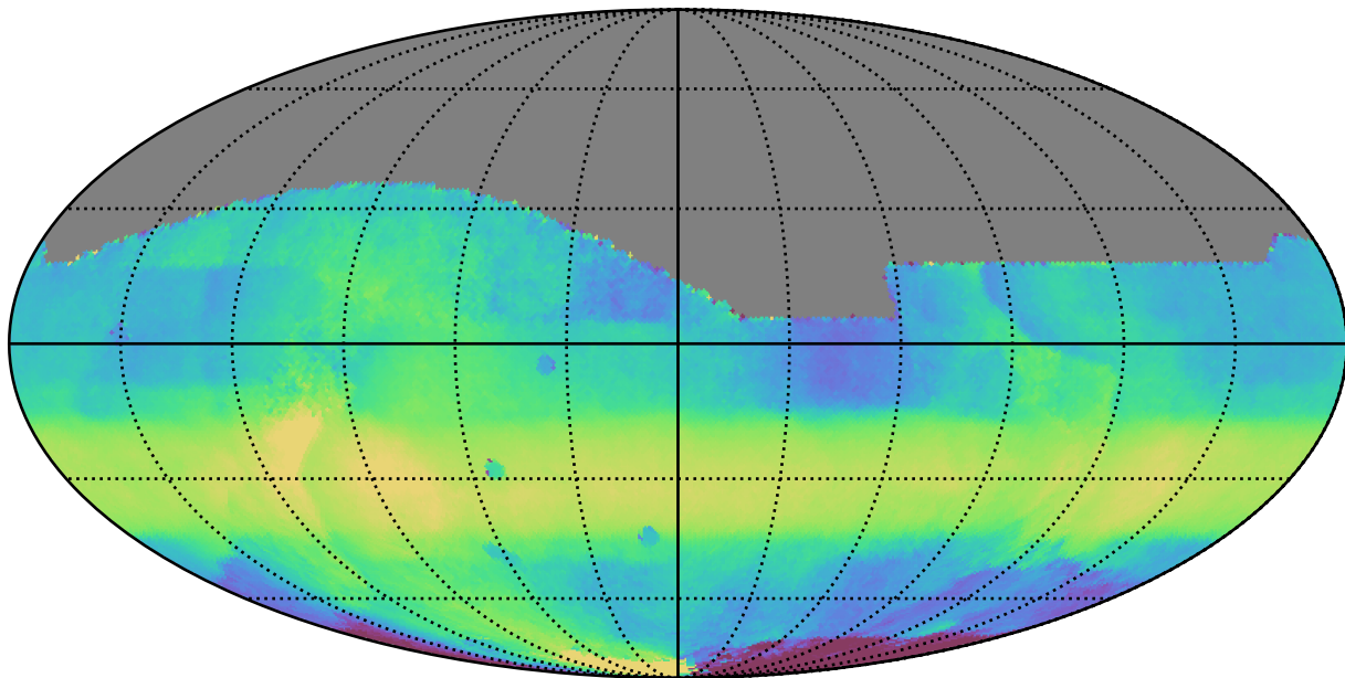
ddf_acor_sf10_lsf40_lsr50_v3.4_10yrs All sky all bands: Median HA
