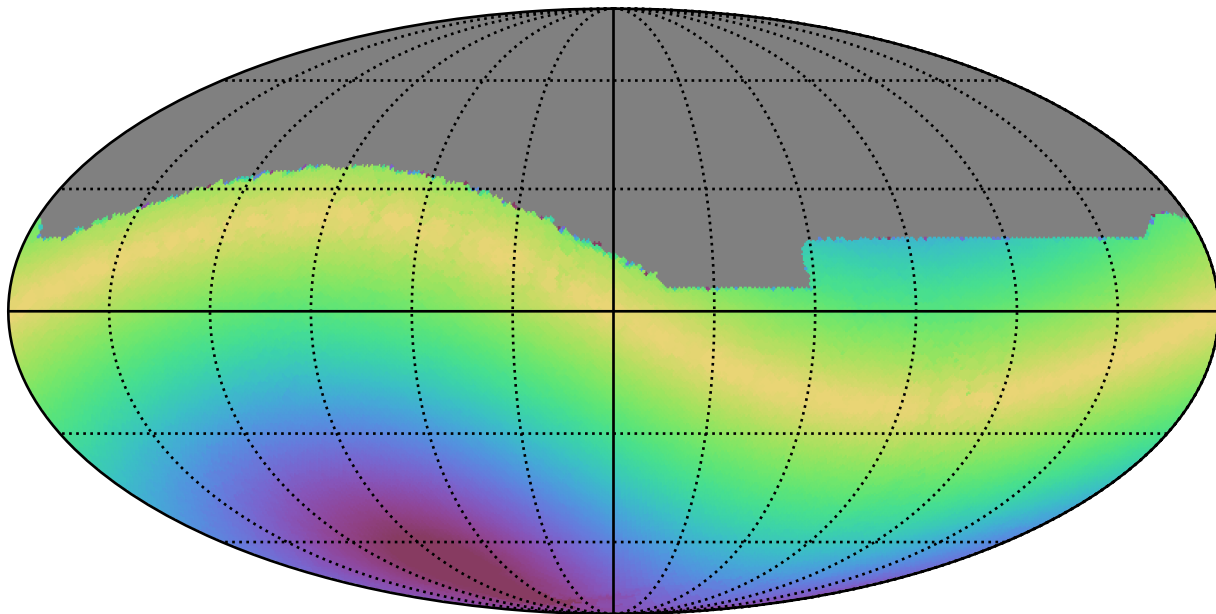
ddf_acor_sf10_lsf40_lsr50_v3.4_10yrs All sky i band: Max solarElong
