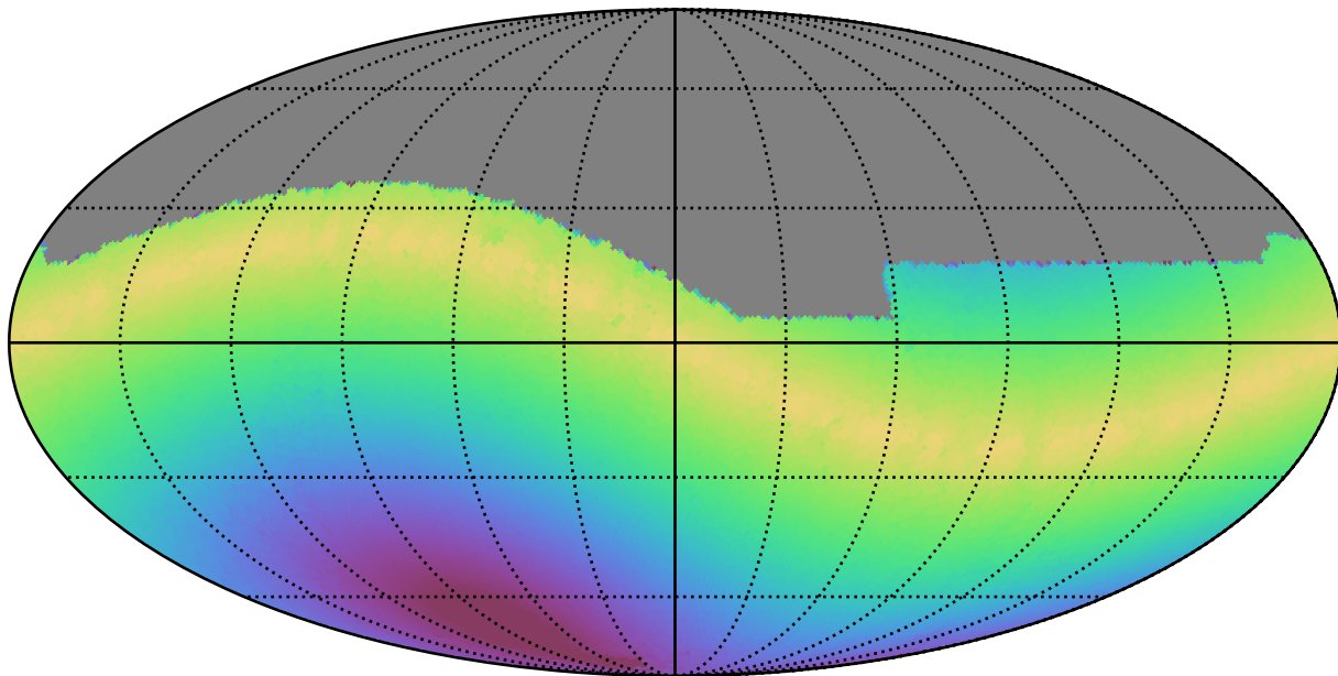
ddf_acor_sf10_lsf40_lsr50_v3.4_10yrs All sky g band: Max solarElong
