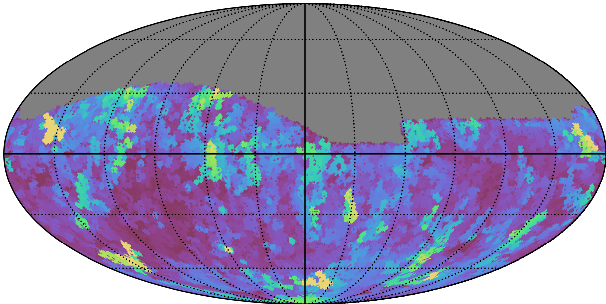
ddf_acor_sf10_lsf40_lsr50_v3.4_10yrs Yr 1 i band: Max seeingEff
