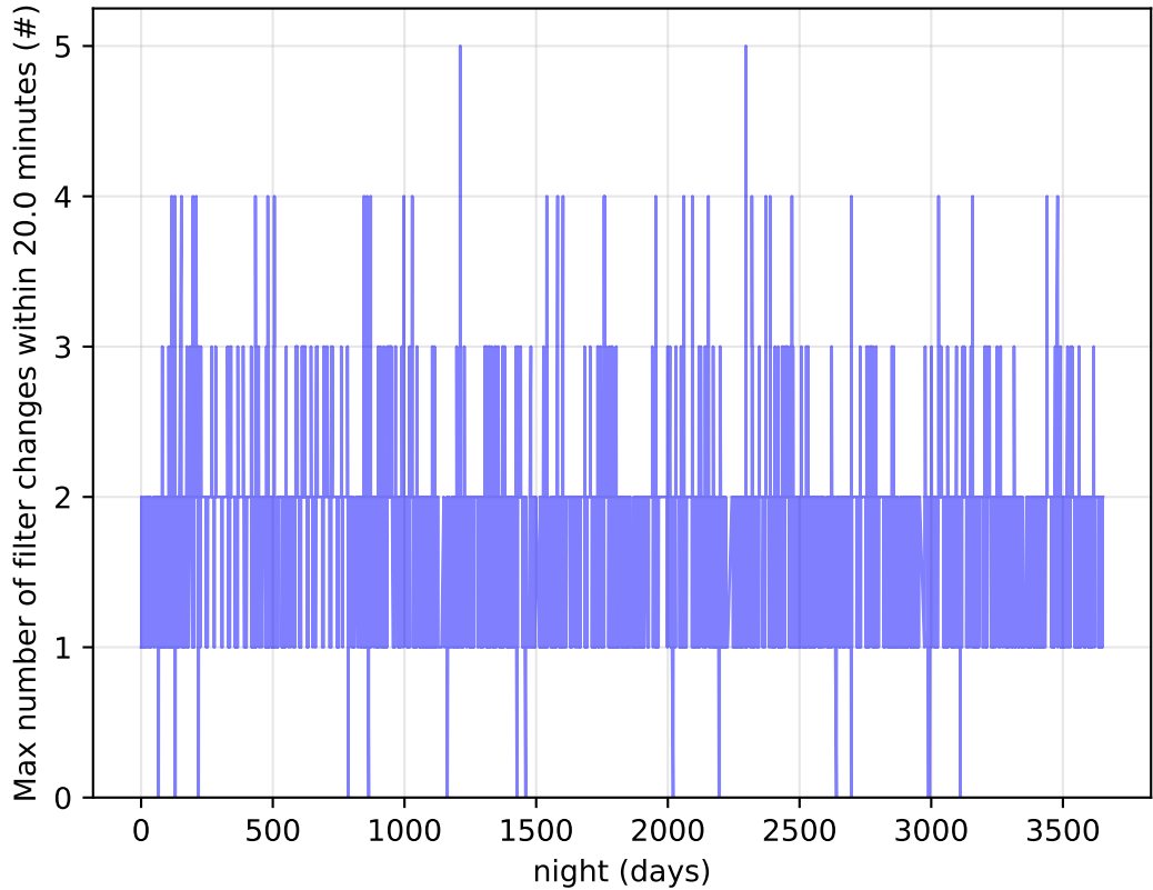
ddf_acor_sf10_Isf40_Isr50_v3.4_10yrs Per Night: Max number of filter changes within 20.0 minutes
