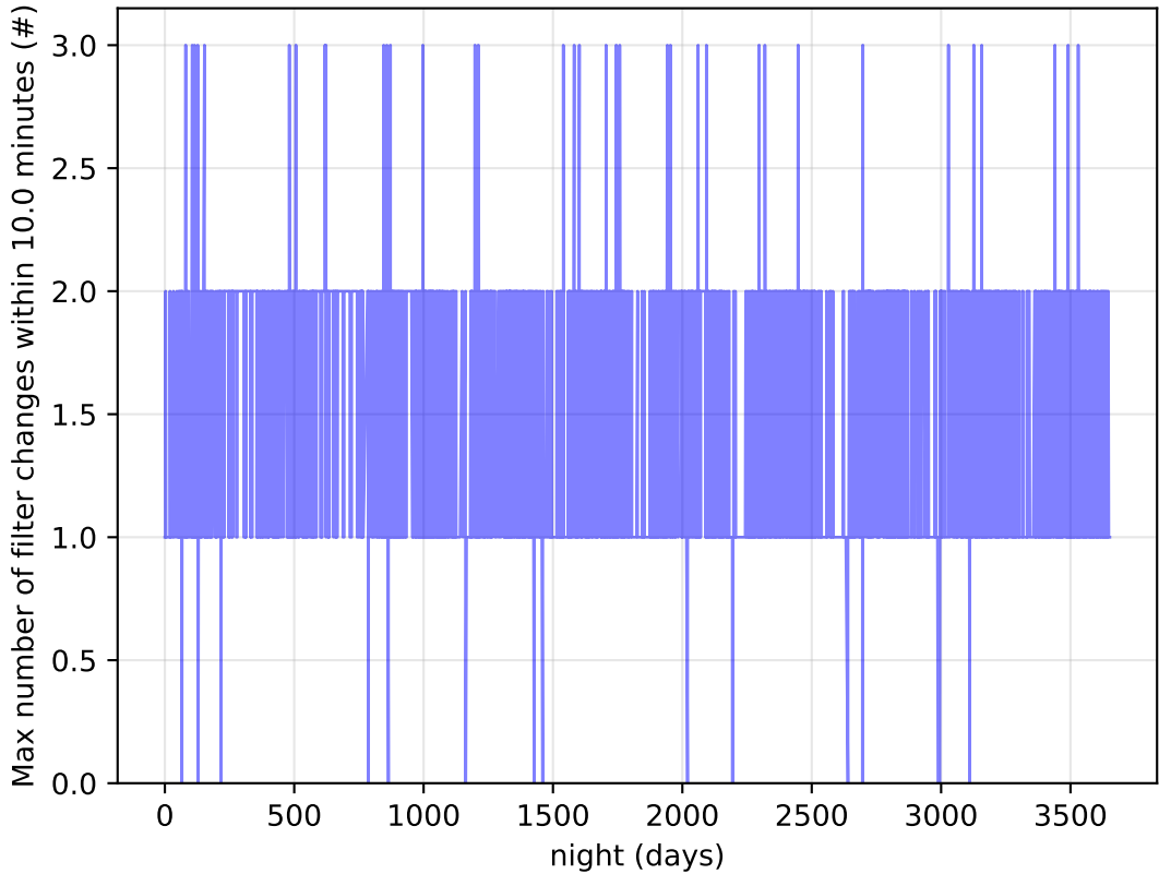
ddf_acor_sf10_Isf40_Isr50_v3.4_10yrs Per Night: Max number of filter changes within 10.0 minutes
