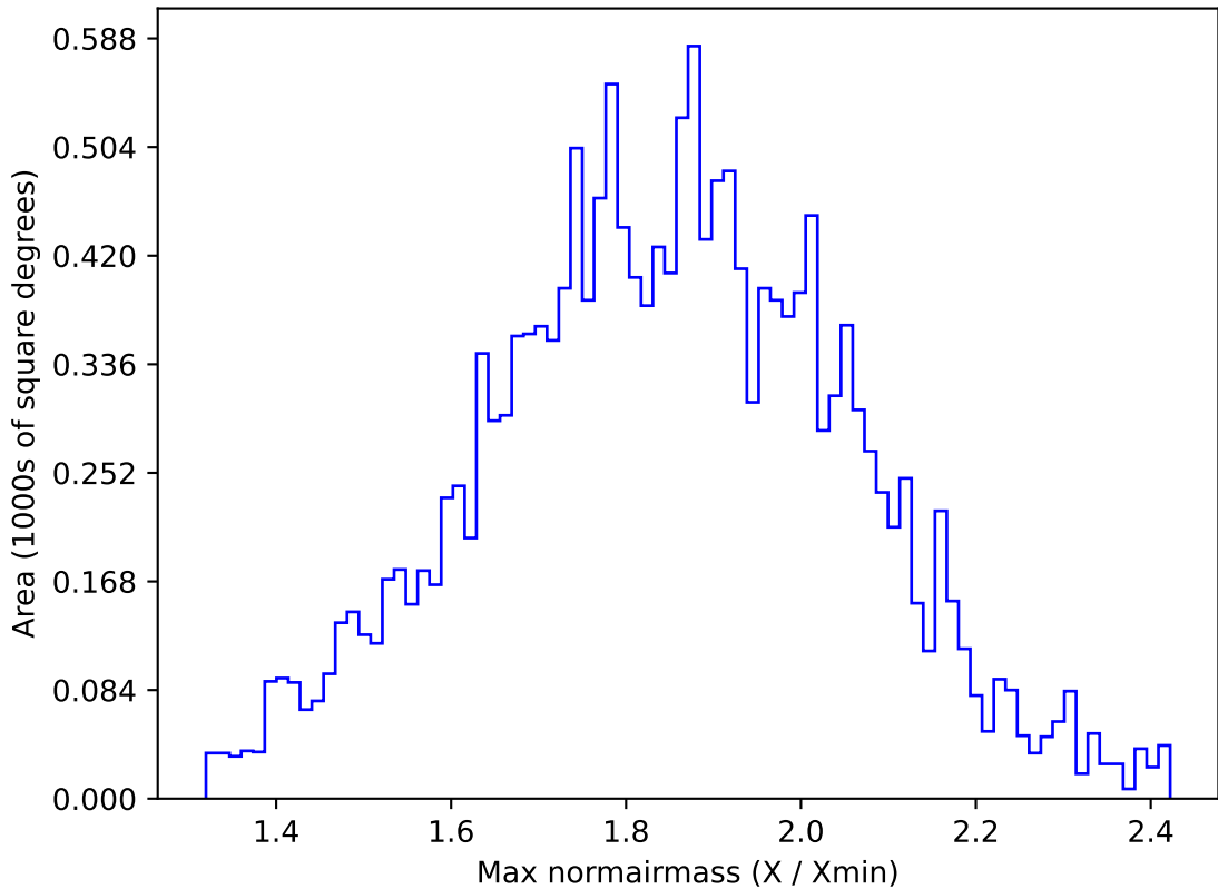
ddf_acor_sf10_lsf40_lsr50_v3.4_10yrs WFD g band: Max normairmass
