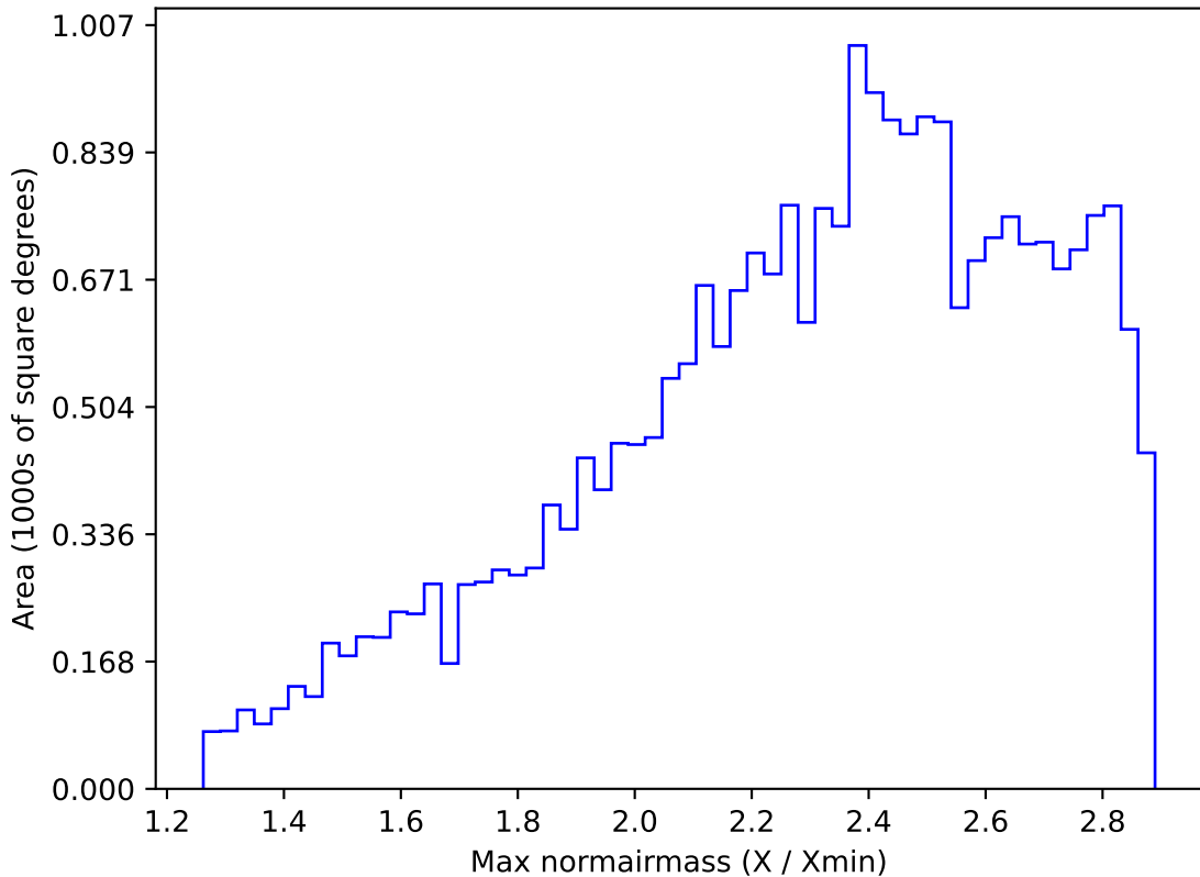
ddf_acor_sf10_lsf40_lsr50_v3.4_10yrs All sky all bands: Max normairmass
