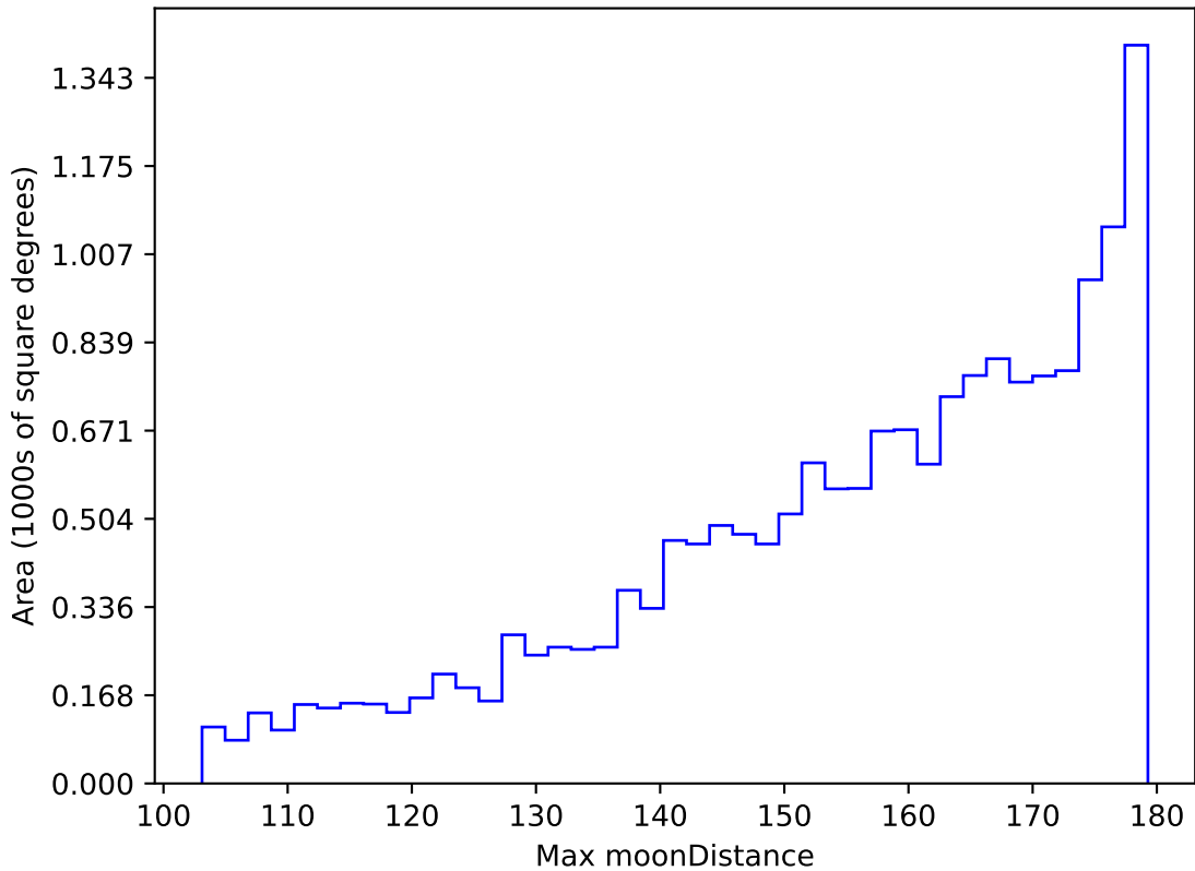
ddf_acor_sf10_lsf40_lsr50_v3.4_10yrs WFD i band: Max moonDistance
