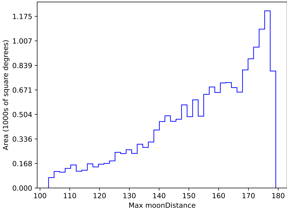
ddf_acor_sf10_lsf40_lsr50_v3.4_10yrs WFD g band: Max moonDistance
