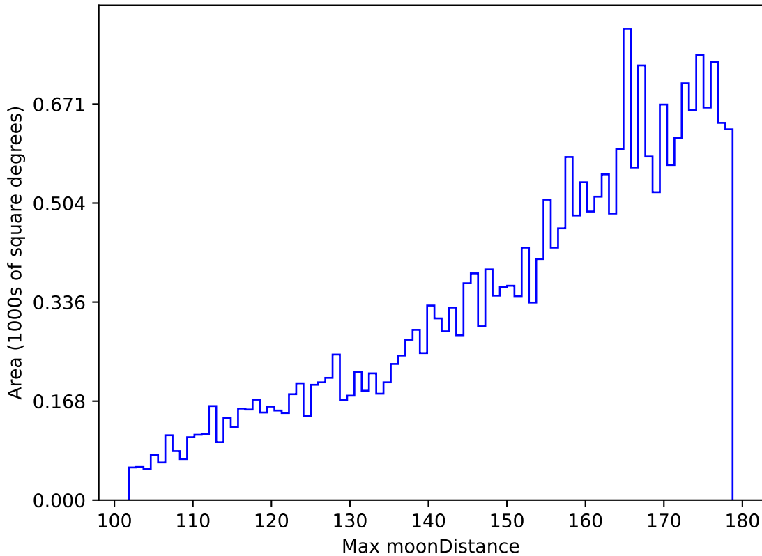
ddf_acor_sf10_lsf40_lsr50_v3.4_10yrs All sky z band: Max moonDistance
