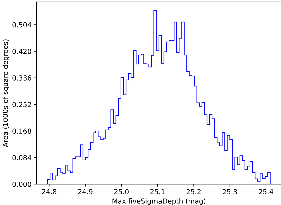
ddf_acor_sf10_lsf40_lsr50_v3.4_10yrs WFD all bands: Max fiveSigmaDepth
