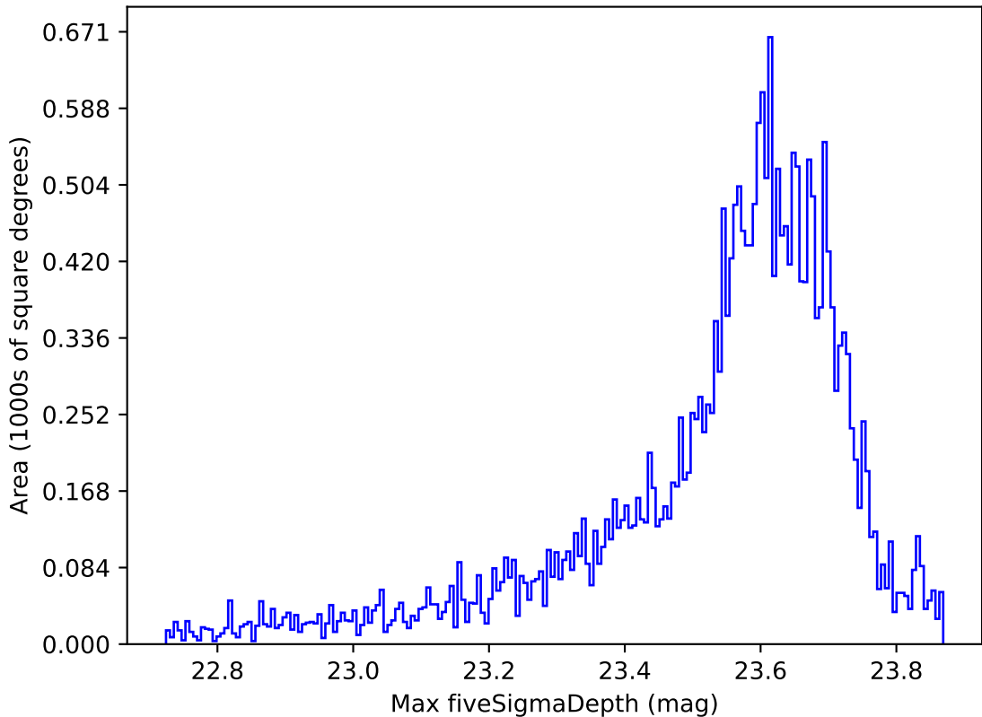
ddf_acor_sf10_lsf40_lsr50_v3.4_10yrs All sky z band: Max fiveSigmaDepth
