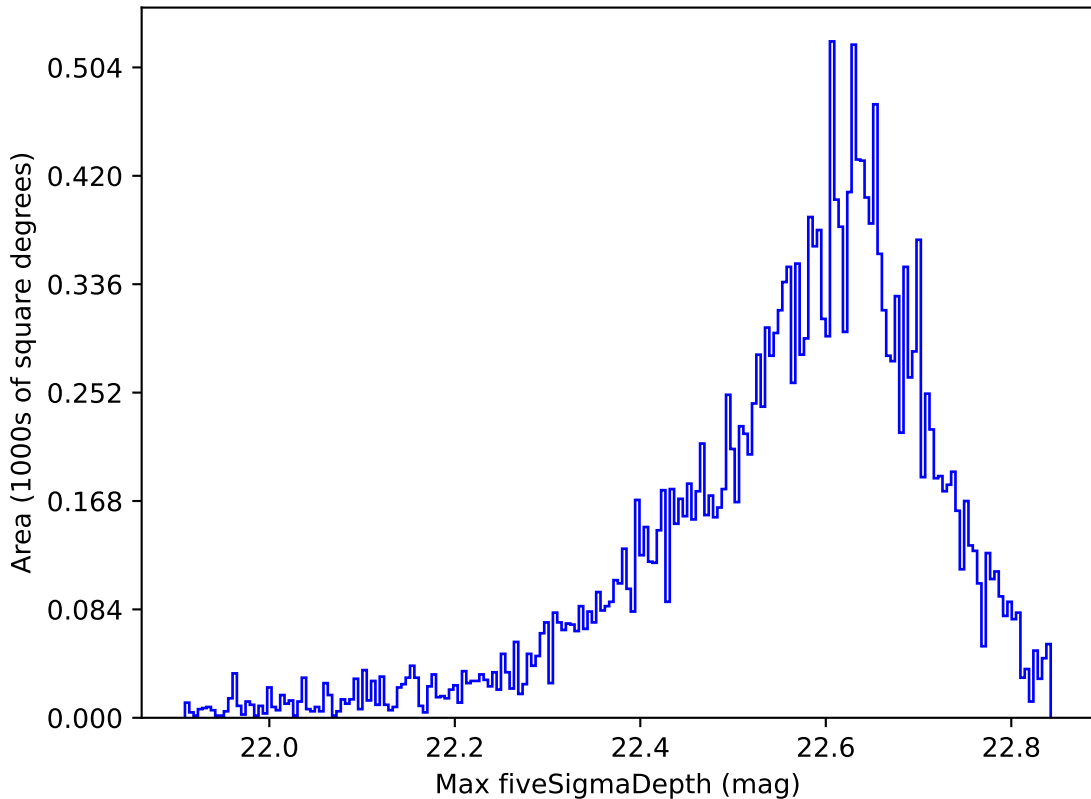
ddf_acor_sf10_lsf40_lsr50_v3.4_10yrs All sky y band: Max fiveSigmaDepth
