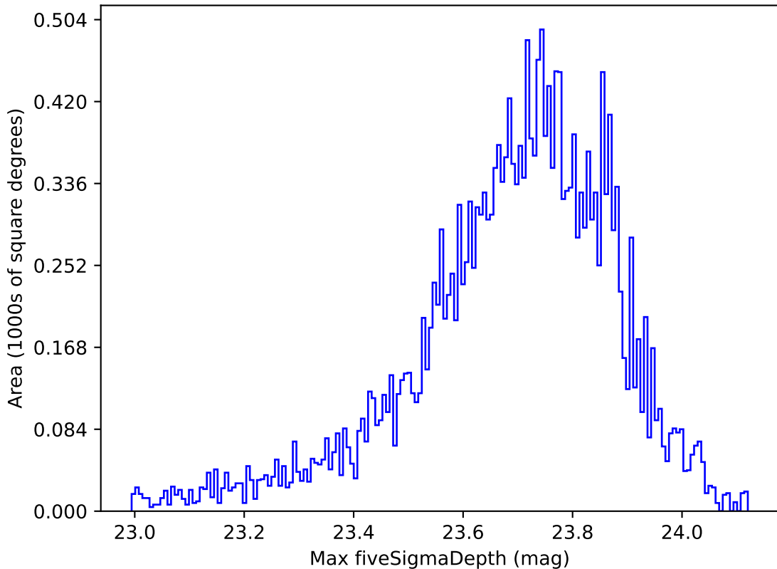
ddf_acor_sf10_ls40_lsr50_v3.4_10yrs All sky u band: Max fiveSigmaDepth
