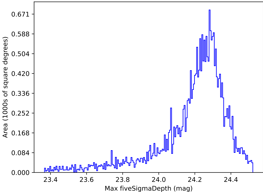
ddf_acor_sf10_lsf40_lsr50_v3.4_10yrs All sky i band: Max fiveSigmaDepth
