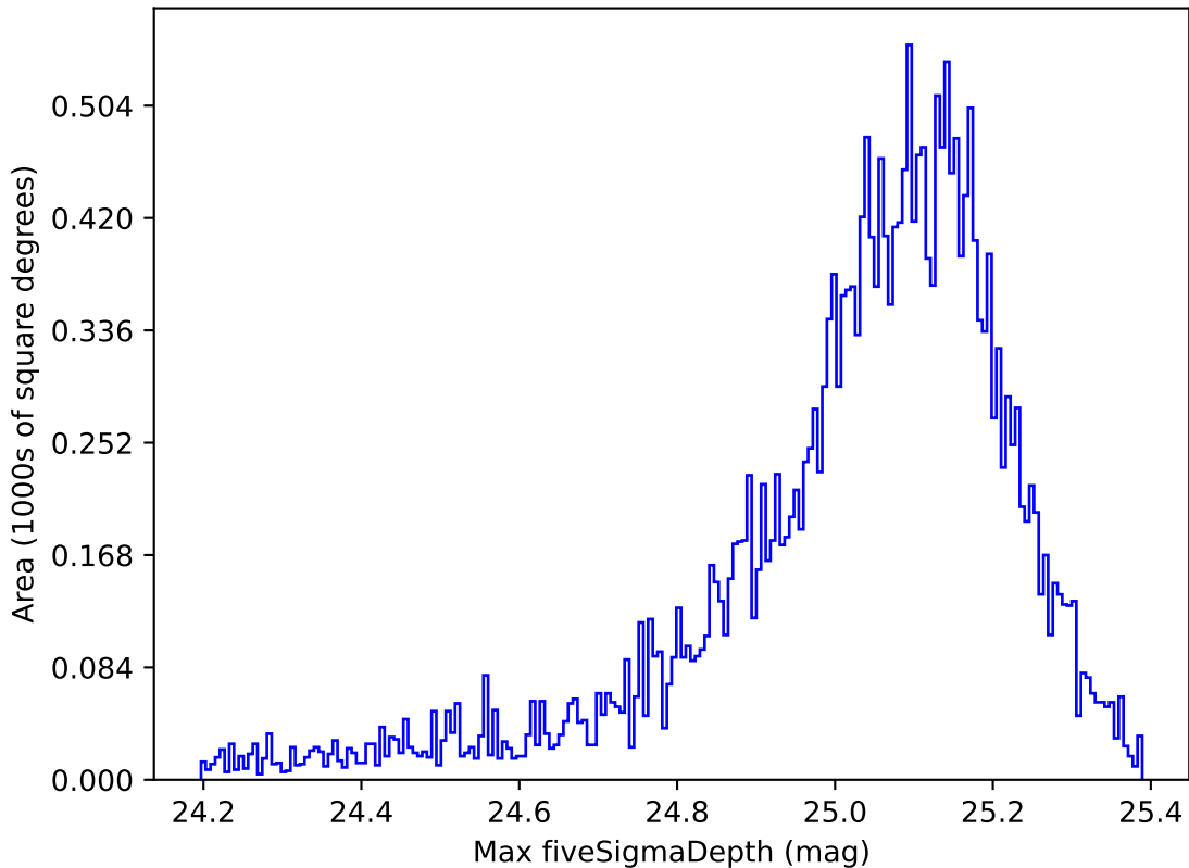
ddf_acor_sf10_ls40_lsr50_v3.4_10yrs All sky g band: Max fiveSigmaDepth
