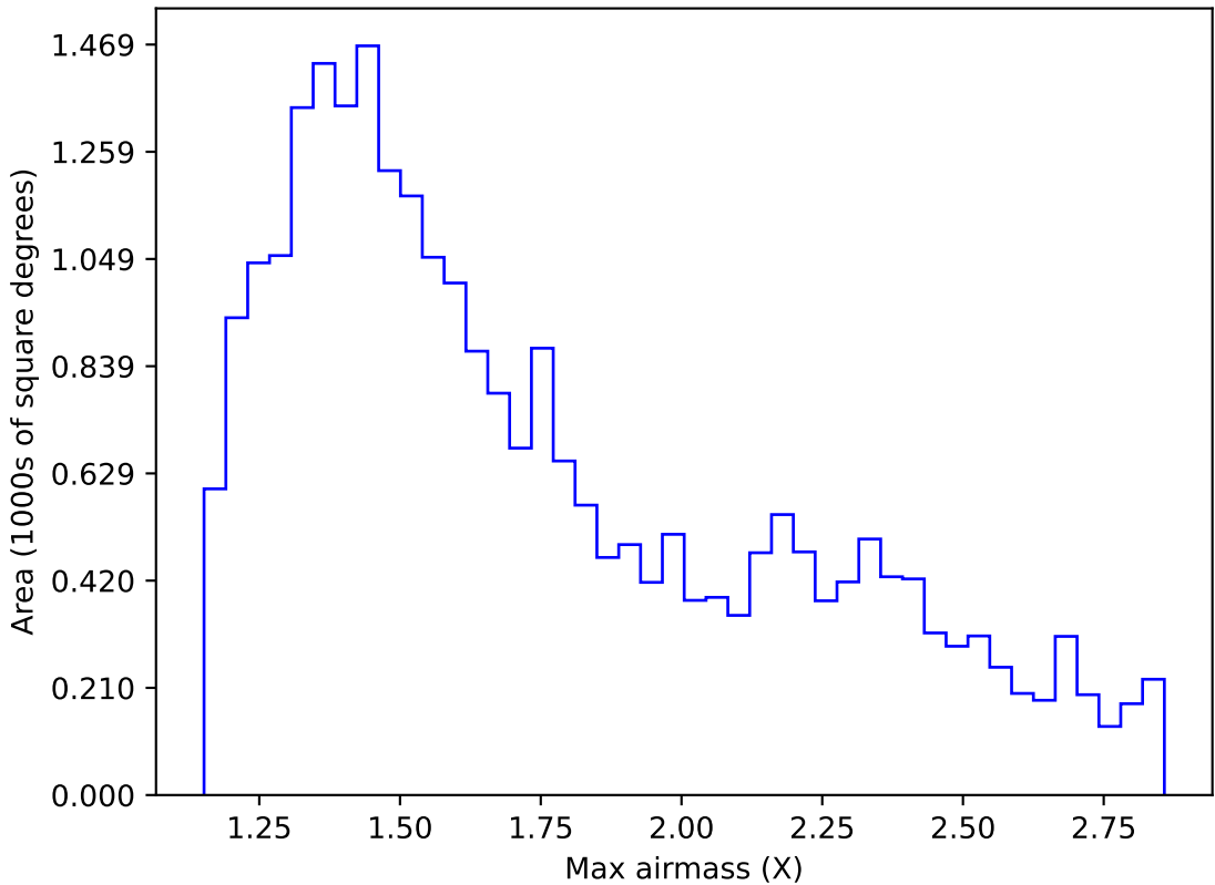
ddf_acor_sf10_lsf40_lsr50_v3.4_10yrs Yr 1 z band: Max airmass
