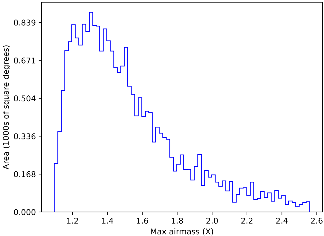
ddf_acor_sf10_lsf40_lsr50_v3.4_10yrs Yr 1 u band: Max airmass
