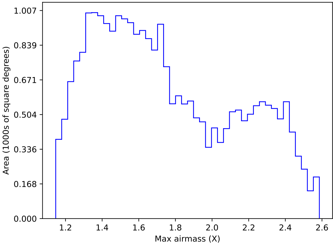
ddf_acor_sf10_lsf40_lsr50_v3.4_10yrs Yr 1 r band: Max airmass
