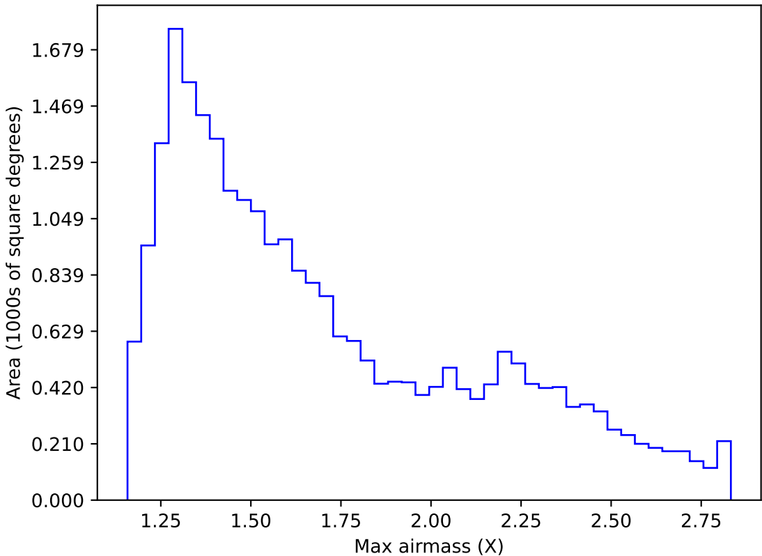
ddf_acor_sf10_lsf40_lsr50_v3.4_10yrs Yr 1 i band: Max airmass
