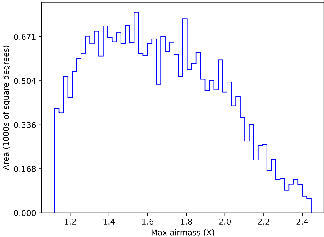
ddf_acor_sf10_lsf40_lsr50_v3.4_10yrs Yr 1 g band: Max airmass
