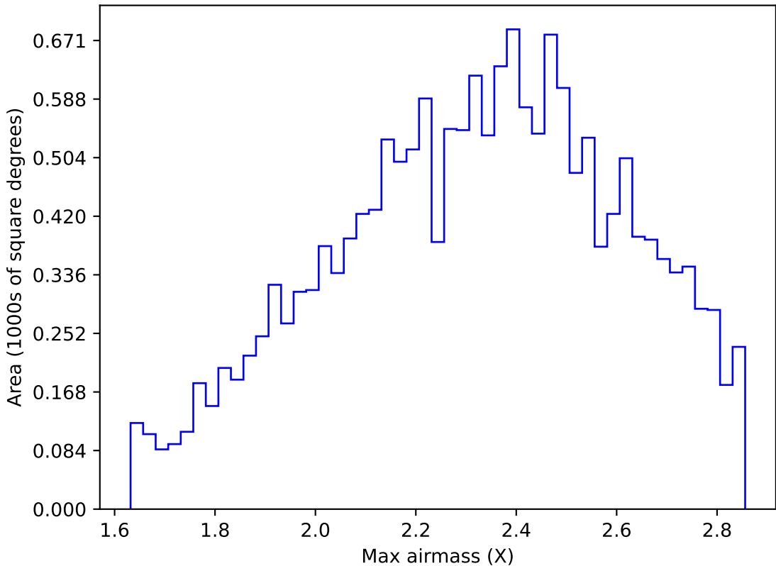
ddf_acor_sf10_ls40_lsr50_v3.4_10yrs WFD y band: Max airmass
