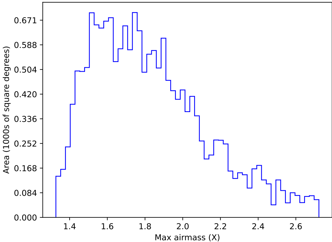
ddf_acor_sf10_lsf40_lsr50_v3.4_10yrs WFD u band: Max airmass
