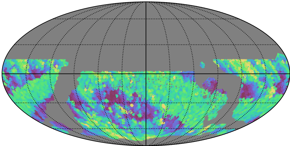
ddf_acor_sf10_lsf40_lsr50_v3.4_10yrs WFD r band: Max airmass
