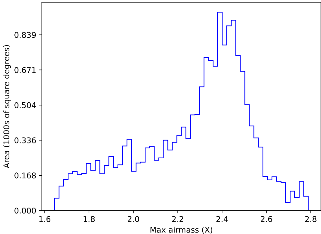
ddf_acor_sf10_lsf40_lsr50_v3.4_10yrs WFD r band: Max airmass
