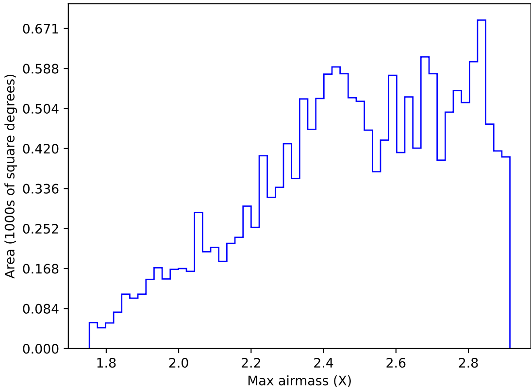
ddf_acor_sf10_lsf40_lsr50_v3.4_10yrs WFD i band: Max airmass
