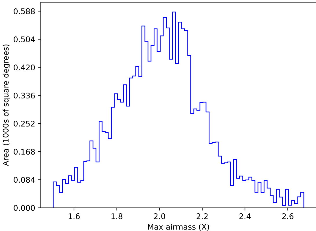
ddf_acor_sf10_ls40_lsr50_v3.4_10yrs WFD g band: Max airmass
