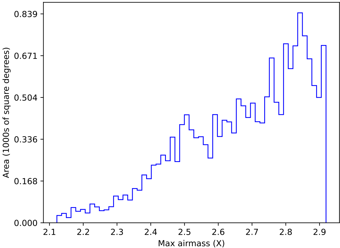
ddf_acor_sf10_lsf40_lsr50_v3.4_10yrs WFD all bands: Max airmass
