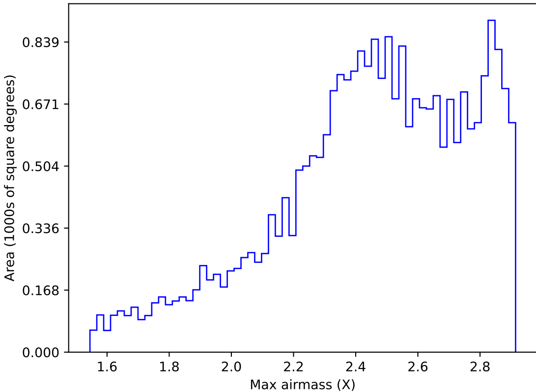
ddf_acor_sf10_lsf40_lsr50_v3.4_10yrs All sky z band: Max airmass
