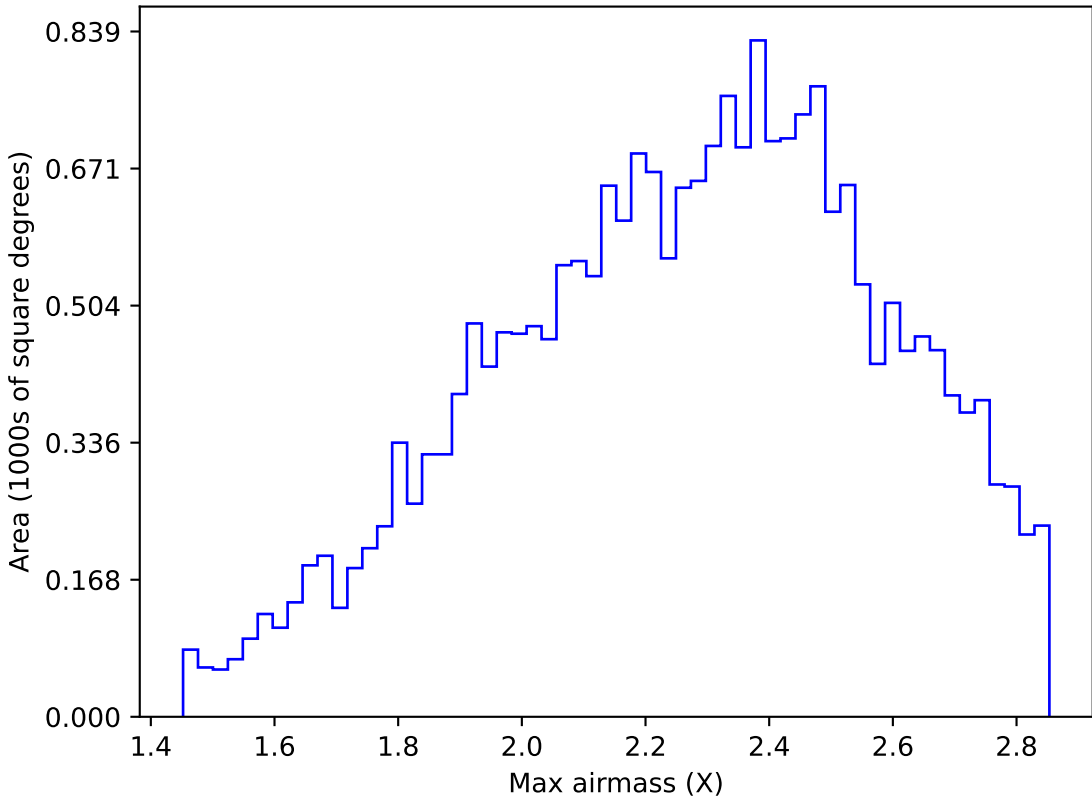
ddf_acor_sf10_lsf40_lsr50_v3.4_10yrs All sky y band: Max airmass
