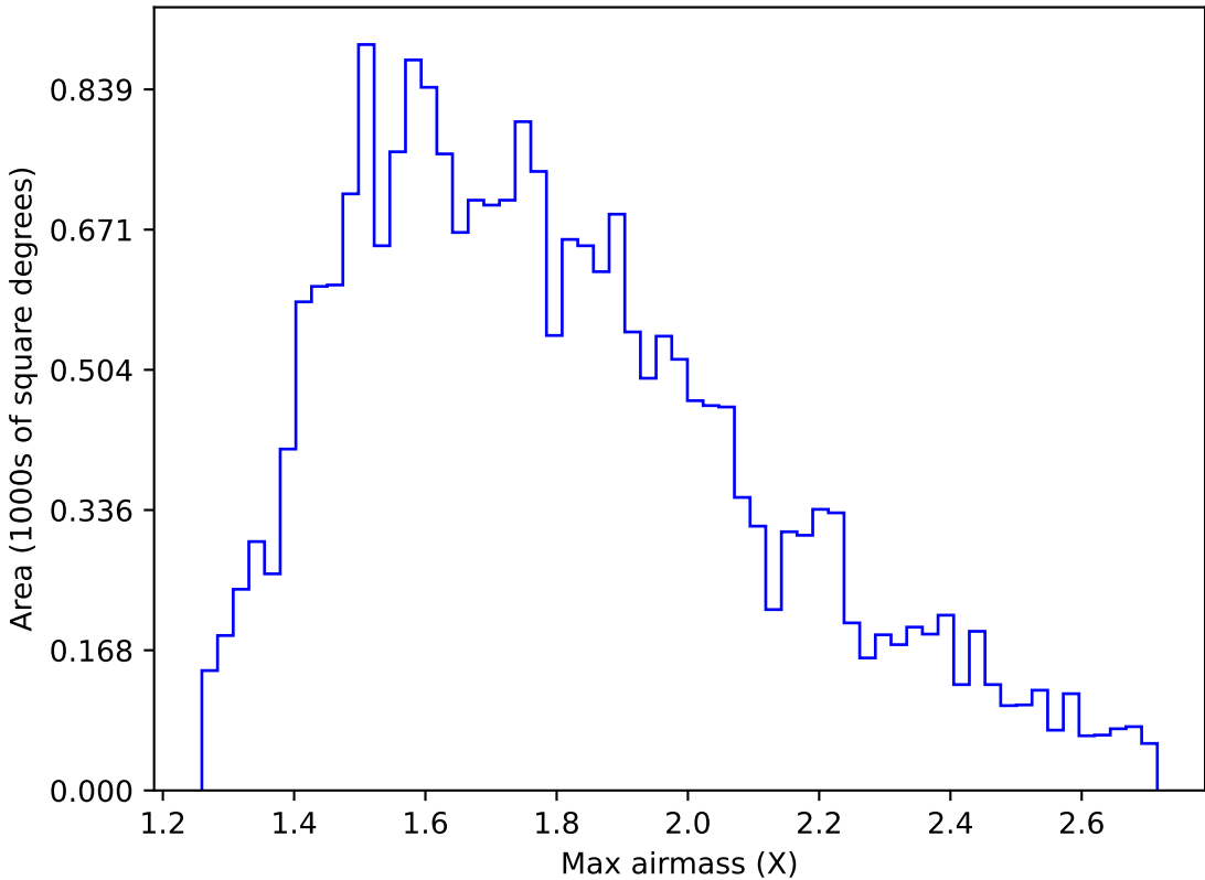
ddf_acor_sf10_lsf40_lsr50_v3.4_10yrs All sky u band: Max airmass
