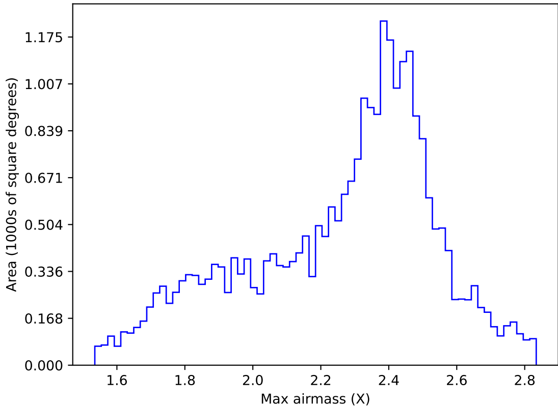
ddf_acor_sf10_lsf40_lsr50_v3.4_10yrs All sky r band: Max airmass
