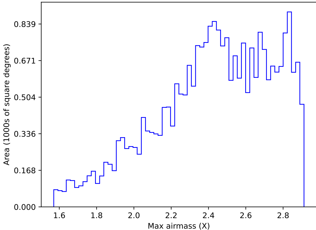
ddf_acor_sf10_lsf40_lsr50_v3.4_10yrs All sky i band: Max airmass
