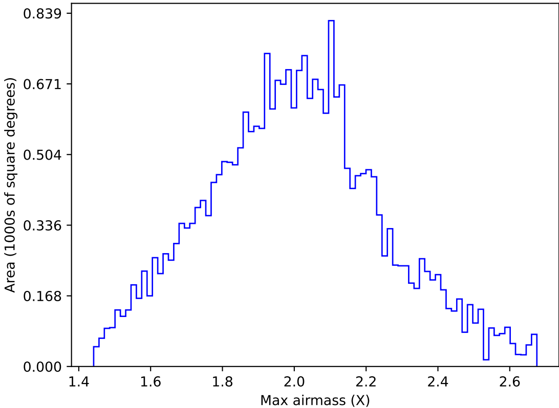
ddf_acor_sf10_lsf40_lsr50_v3.4_10yrs All sky g band: Max airmass
