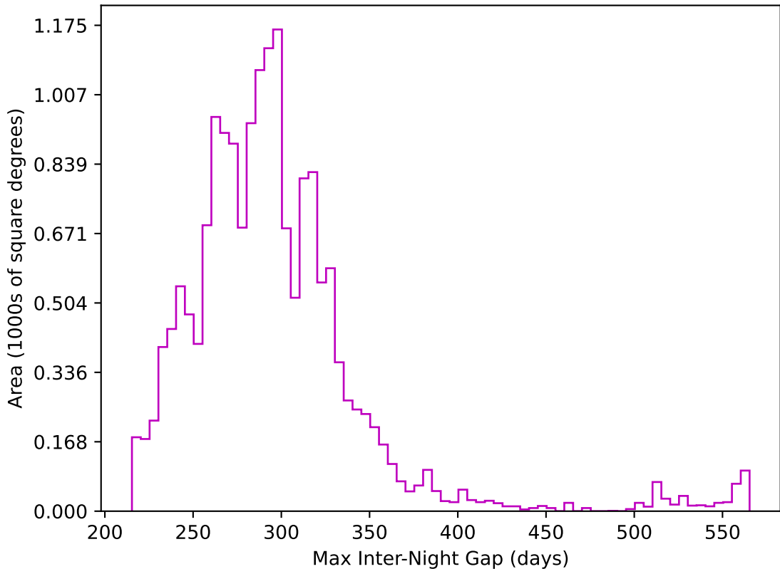
ddf_acor_sf10_lsf40_lsr50_v3.4_10yrs WFD z band: Max Inter-Night Gap
