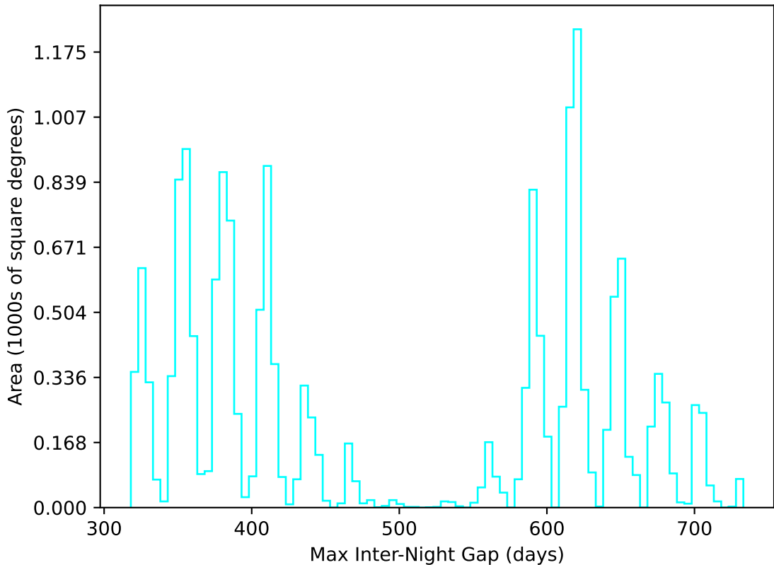
ddf_acor_sf10_lsf40_lsr50_v3.4_10yrs WFD u band: Max Inter-Night Gap
