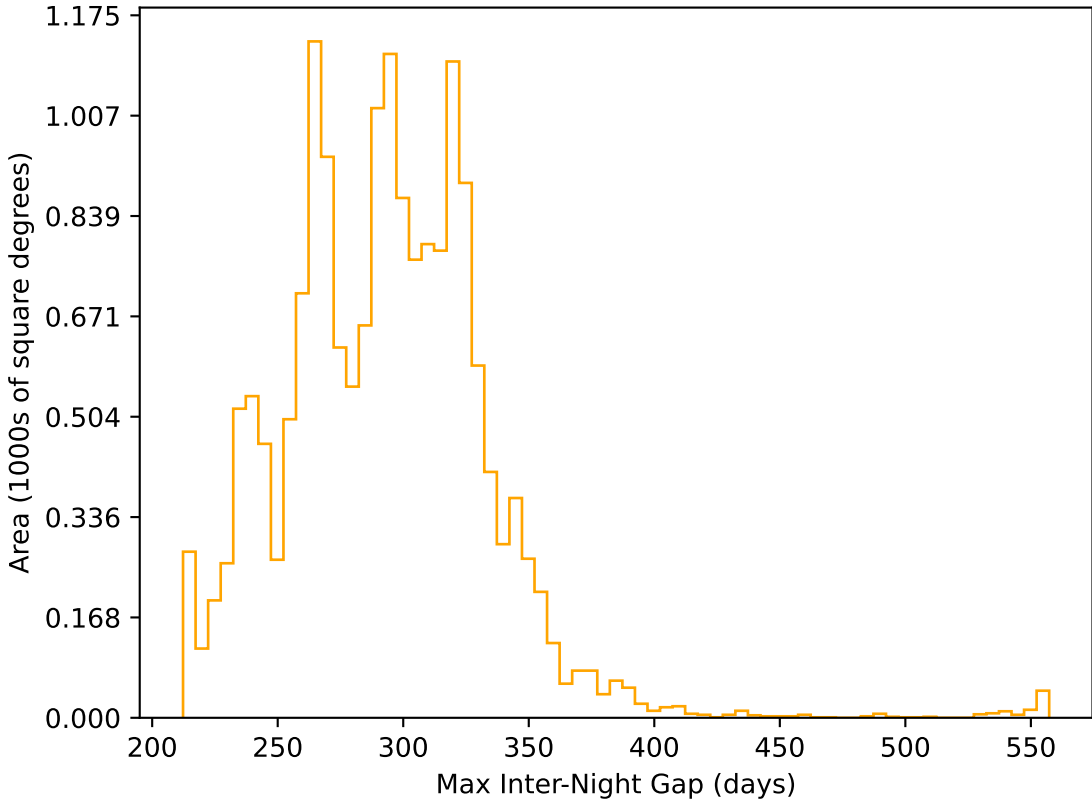
ddf_acor_sf10_lsf40_lsr50_v3.4_10yrs WFD r band: Max Inter-Night Gap
