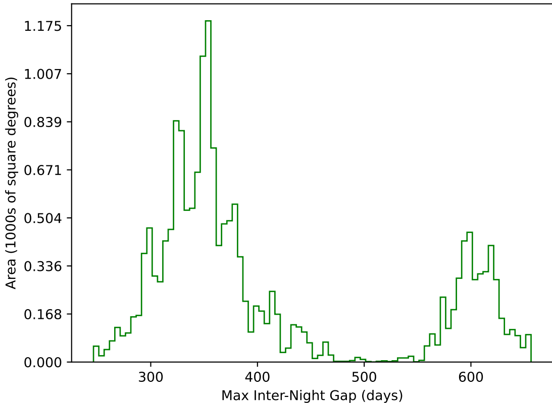
ddf_acor_sf10_lsf40_lsr50_v3.4_10yrs WFD g band: Max Inter-Night Gap
