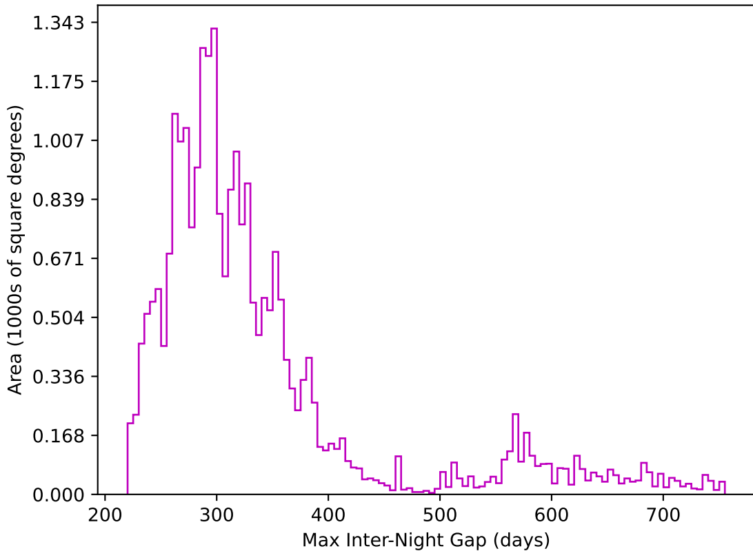
ddf_acor_sf10_lsf40_lsr50_v3.4_10yrs All sky z band: Max Inter-Night Gap
