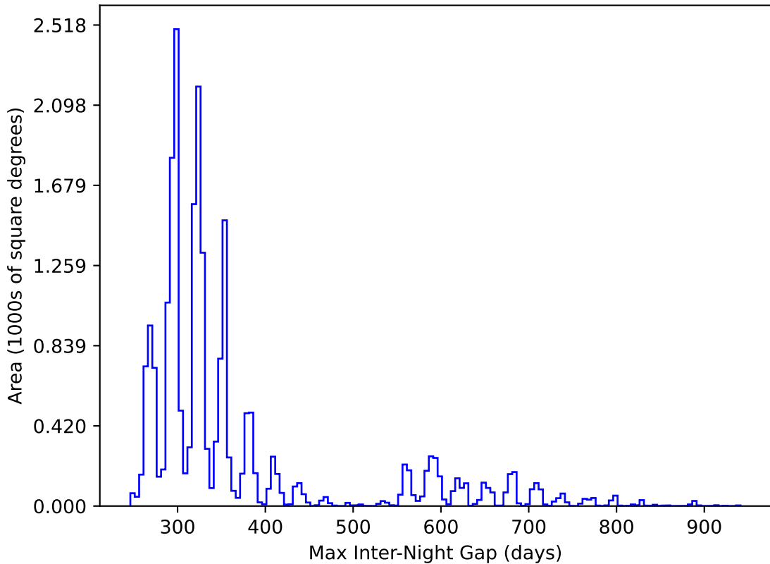
ddf_acor_sf10_lsf40_lsr50_v3.4_10yrs All sky y band: Max Inter-Night Gap
