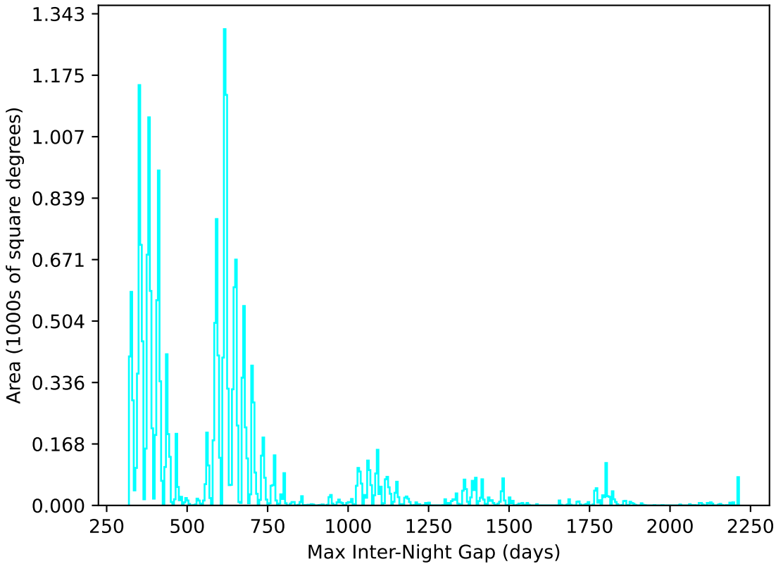
ddf_acor_sf10_ls40_lsr50_v3.4_10yrs All sky u band: Max Inter-Night Gap
