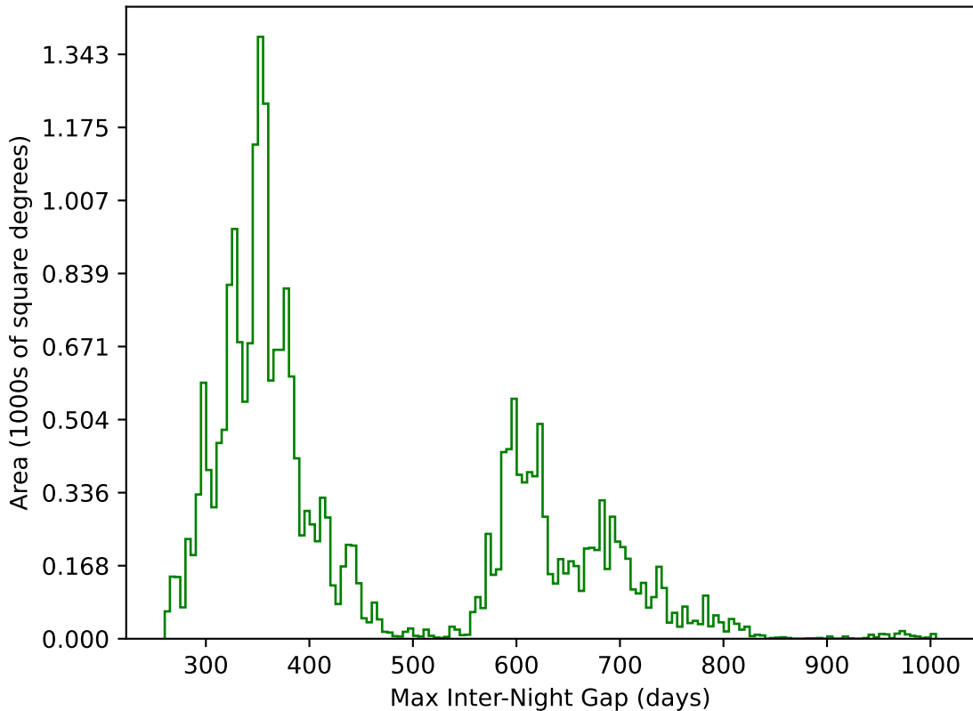
ddf_acor_sf10_lsf40_lsr50_v3.4_10yrs All sky g band: Max Inter-Night Gap
